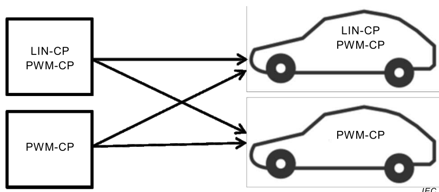
Figure D.8 – Energy transfer between different charging stations and EVs that are equipped with accessories according to IEC 62196-2
